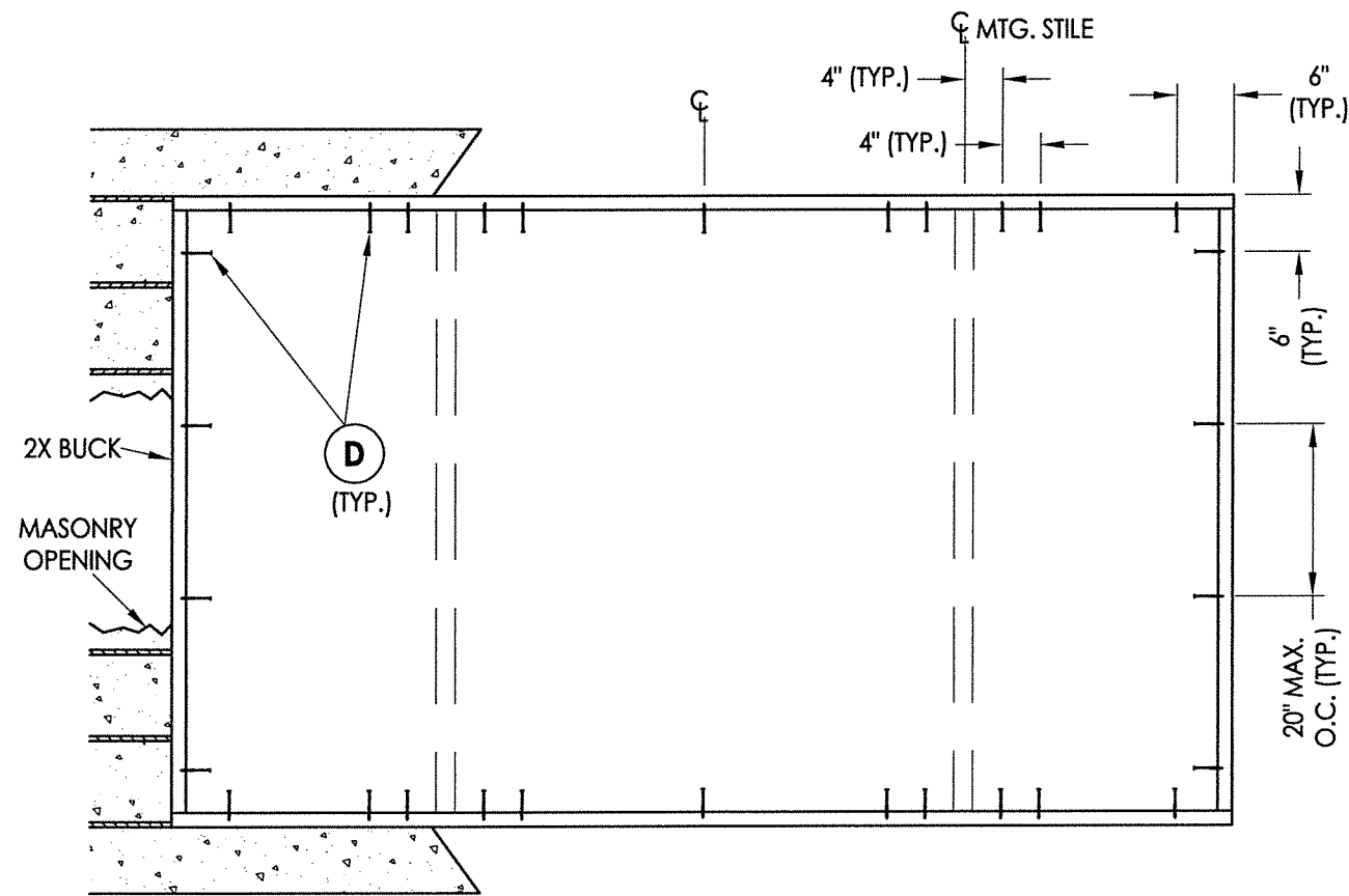
2X BUCK ANCHORING
