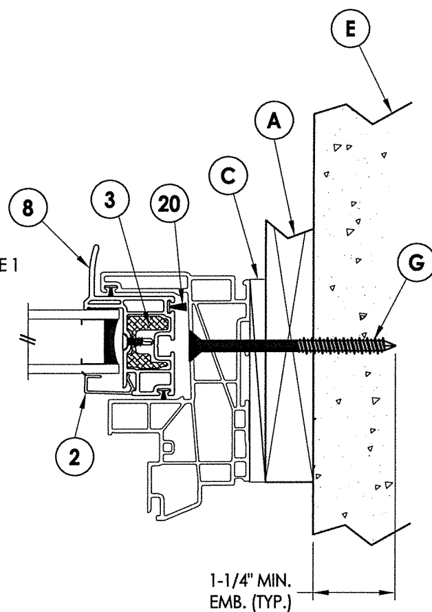
2 HORIZONTAL CROSS SECTION 2 1X Buck Masonry Construction
