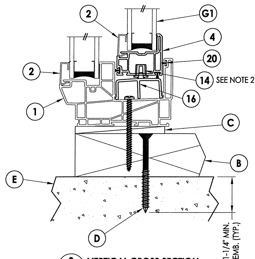
3 VERTICAL CROSS SECTION 2 2X Buck Masonry Construction
