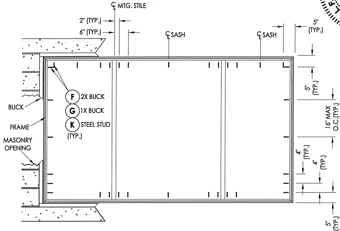
FRAME ANCHORING
