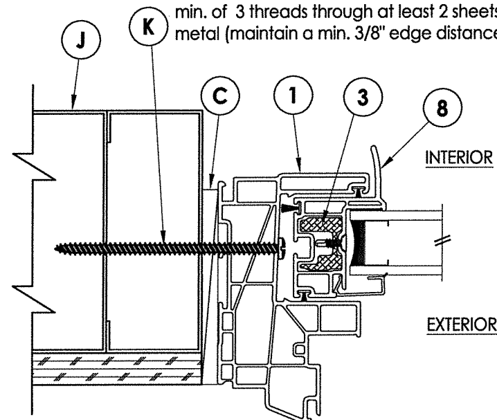
4 2 HORIZONTAL CROSS SECTION
