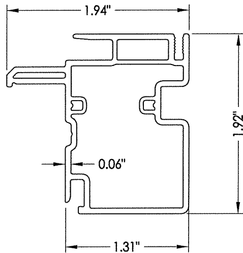
6 MEETING STILE
