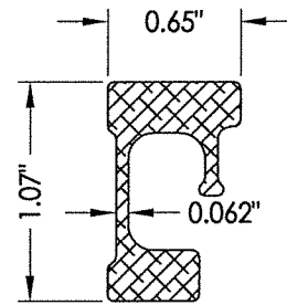
10 LOCK STILE REINFORCEMENT
